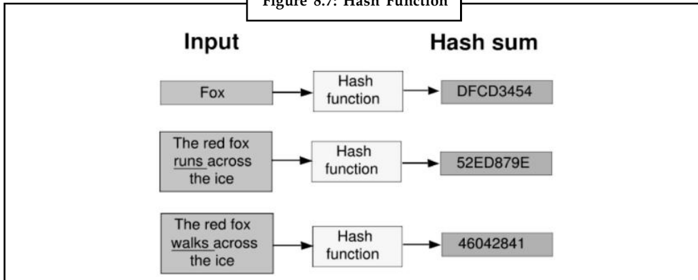
Figure 8.7: Hash Function
